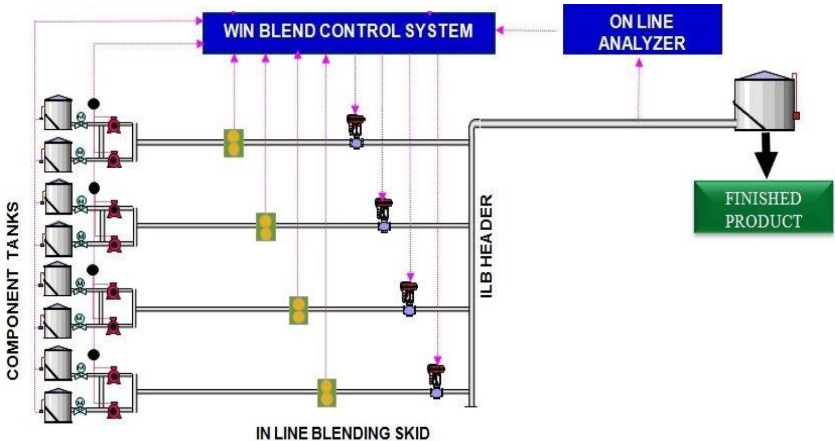
Fuel Blending System – Schematic Diagram (Source: FMC Technologies)
